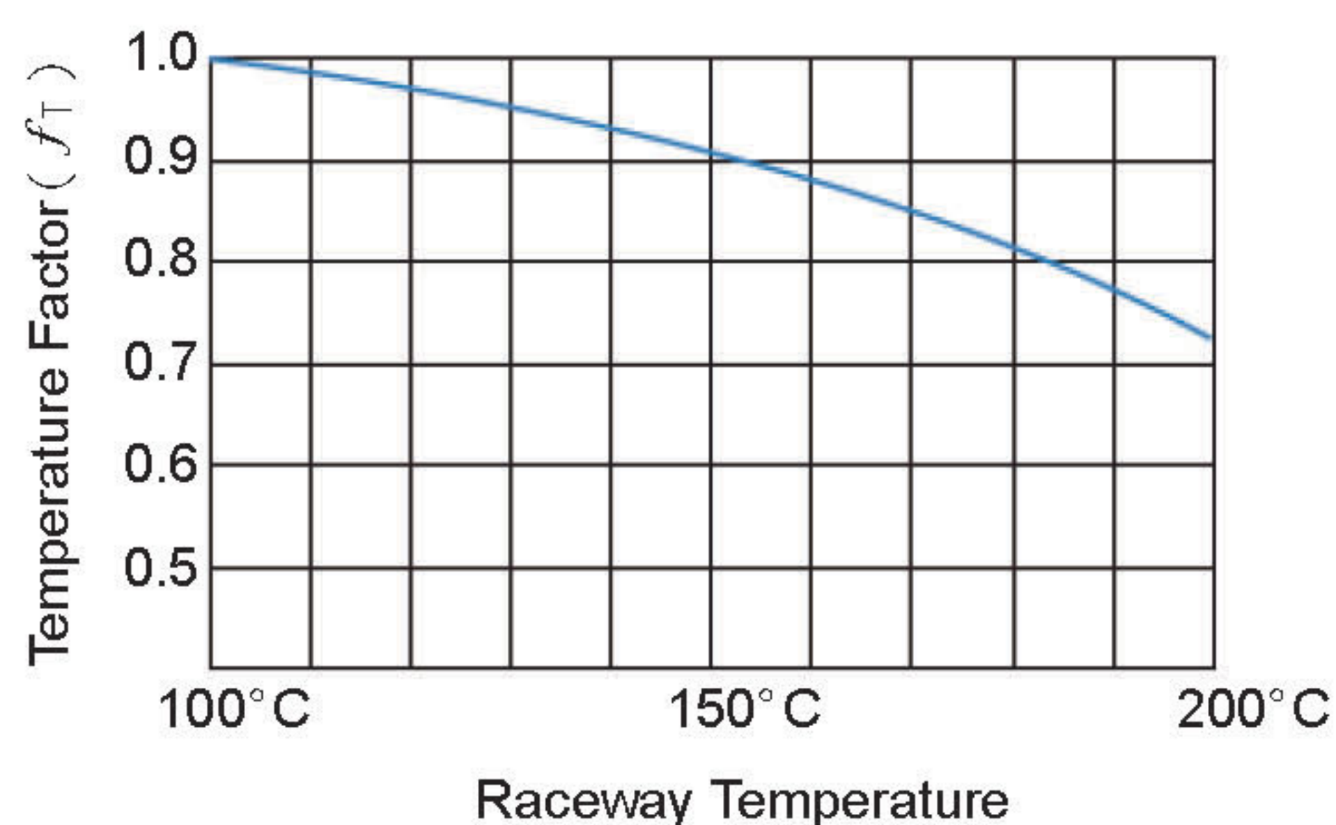
Fig 2.2.2 Temperature Factor ( f_T )
